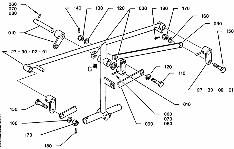
ENSEMBLE PYLONE - RENVOI SUPERIEUR PYLON ASSEMBLY - UPPER BELLCRANK
